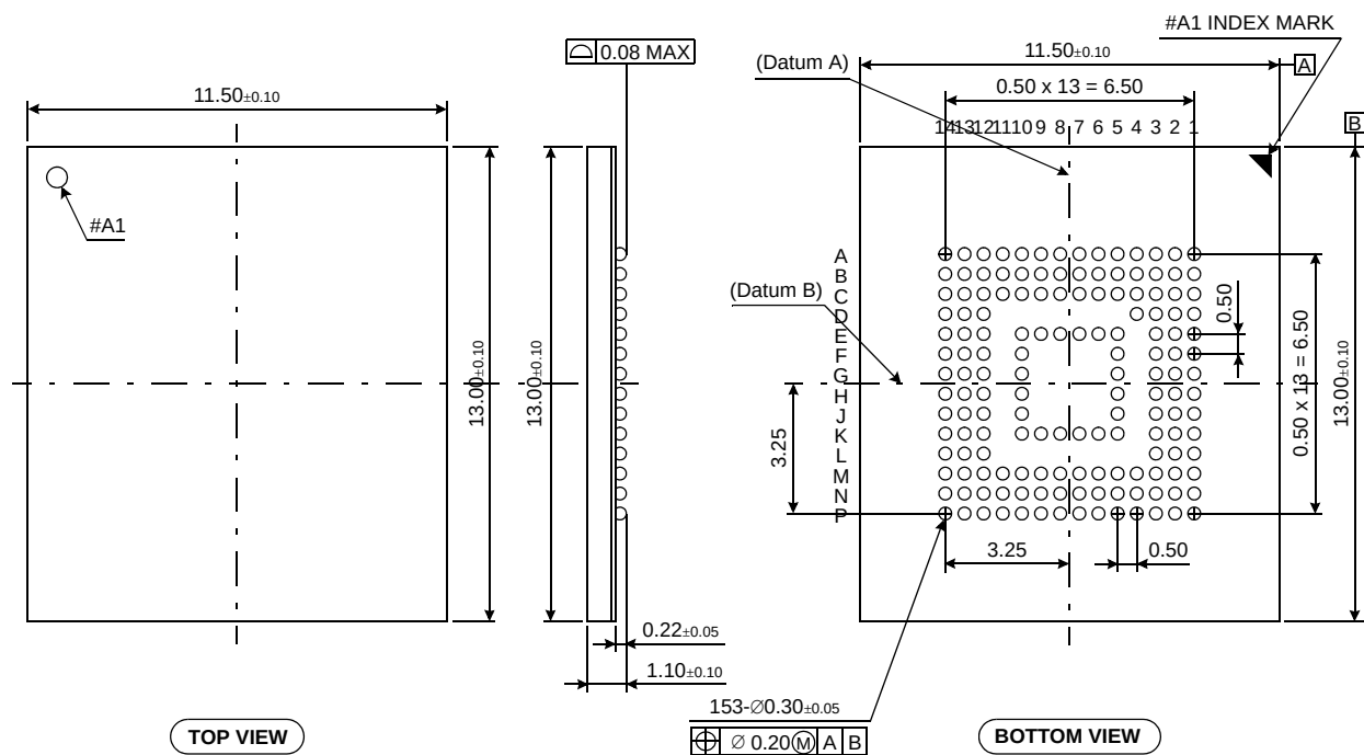
Figure 3. Package Dimension
