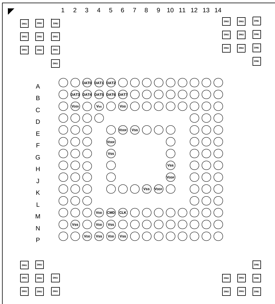
Figure 1. 153-FBGA
