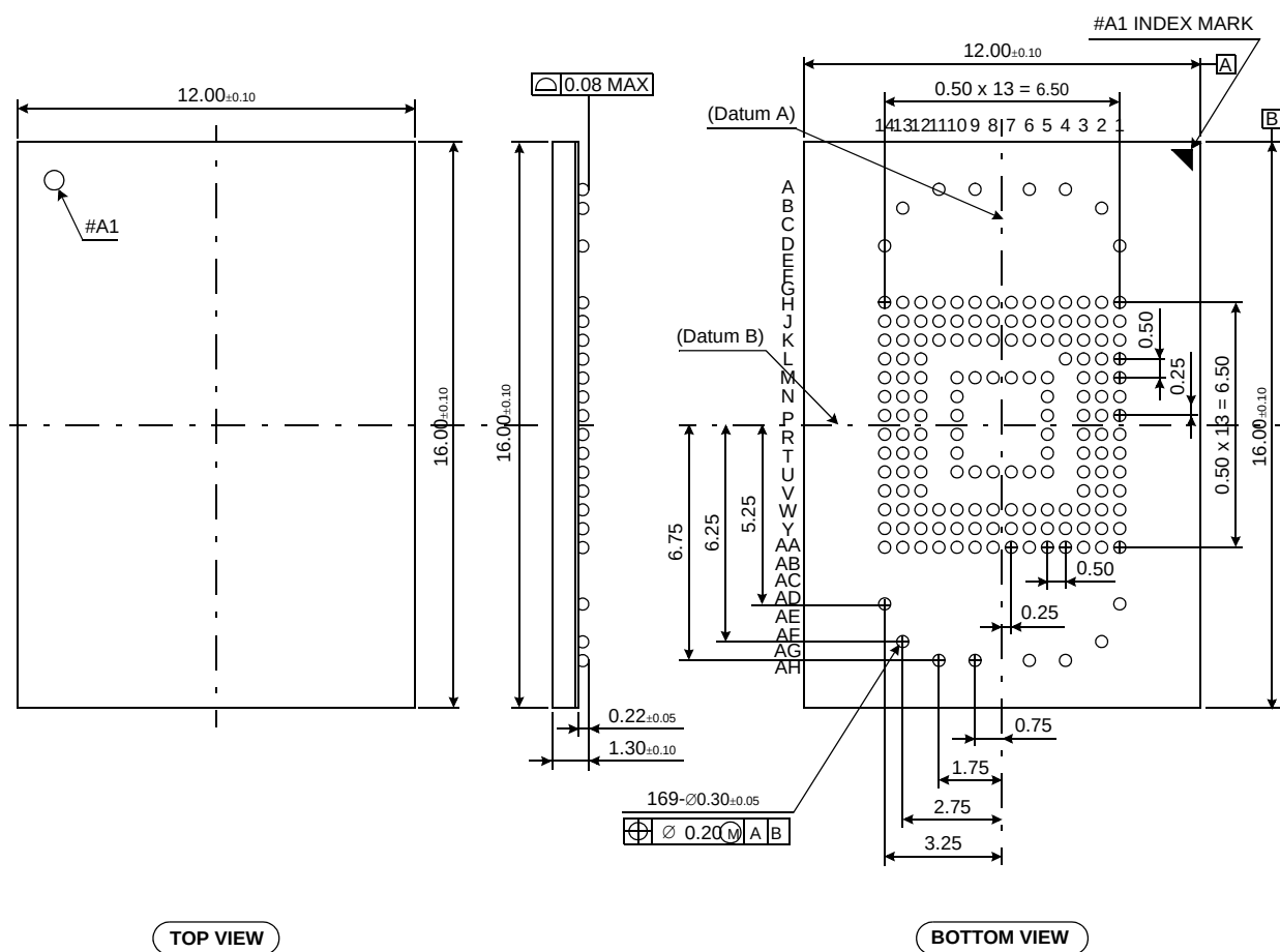
Figure 4. Package Dimension
