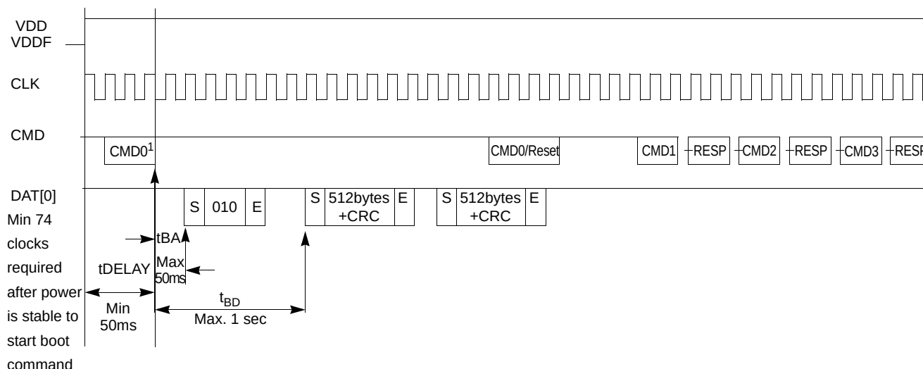
Figure 8. MultiMediaCard state diagram &amp; timing (alternative boot mode)
