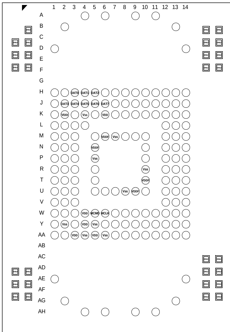
Figure 2. 169-FBGA
