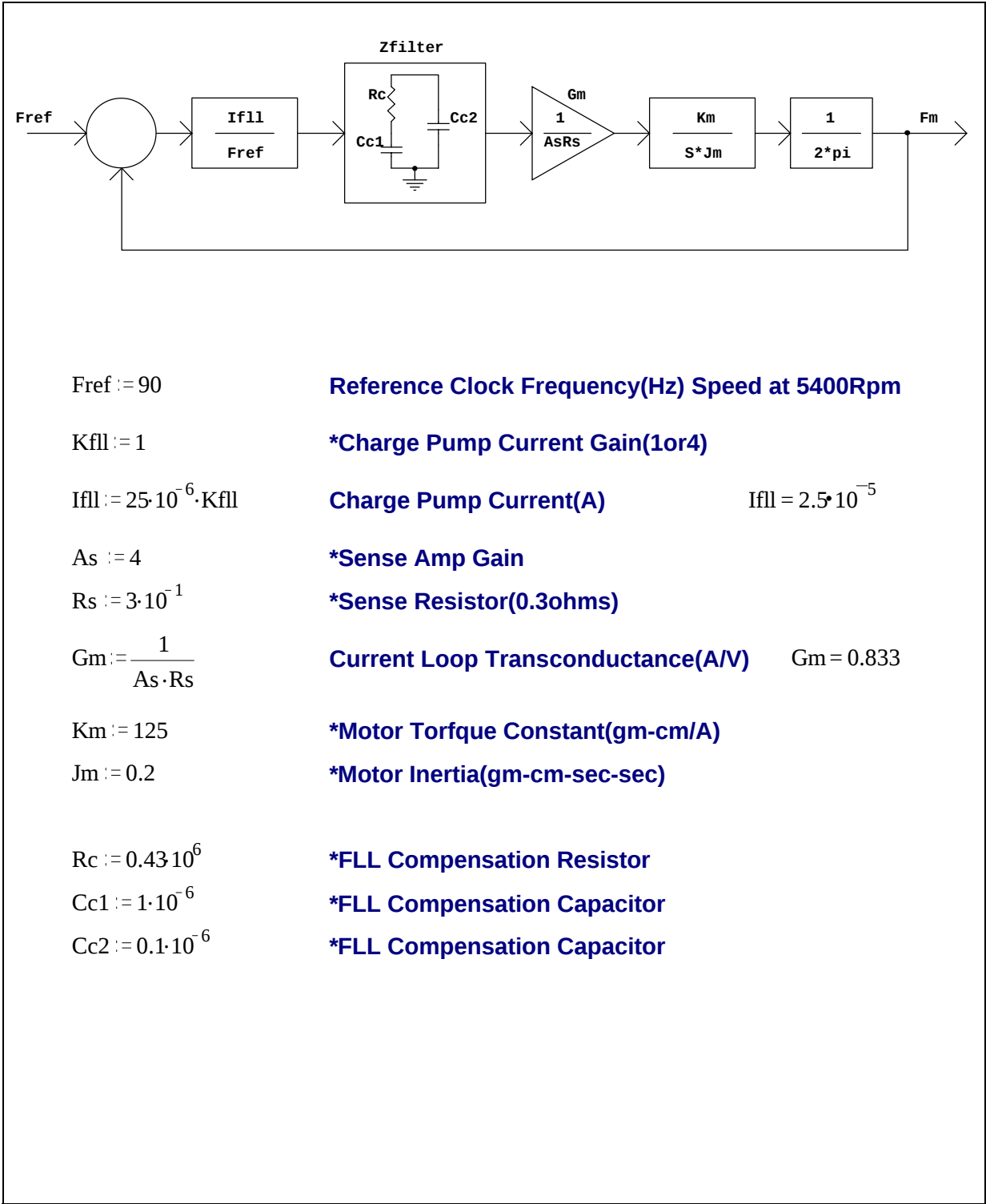
Figure 36. Spindle Speed Control Loop
