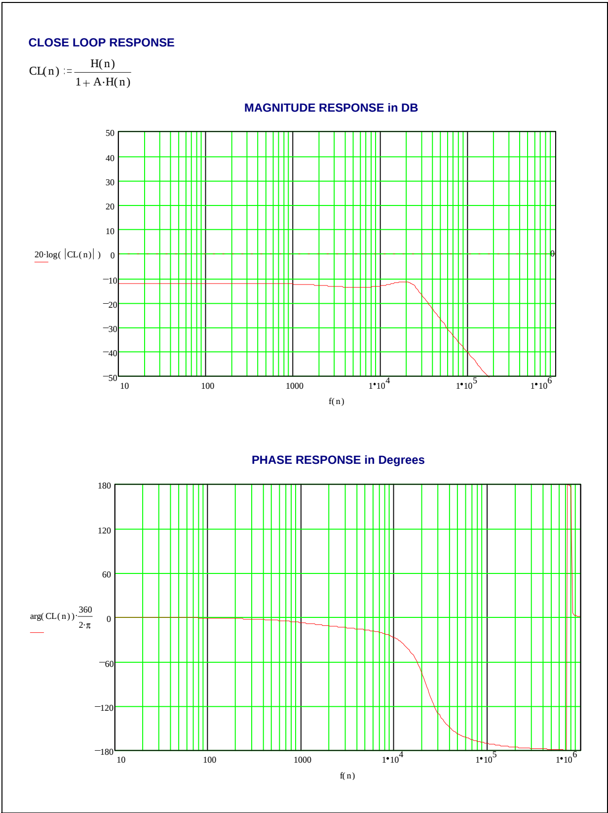
Figure 35c. Mathcad Analisys of the Spindle Current Control Loop
